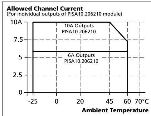
Fig. 19-2 De-rating PISA10.206210
